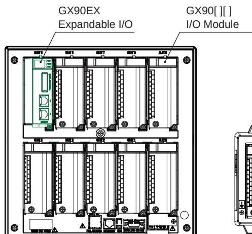
GX20 Configuration example (maximum)
